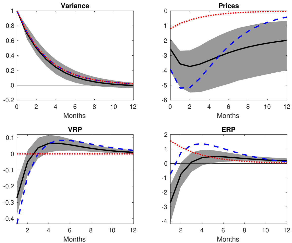
Figure 3: Impulse responses: data vs model. We plot the behavior of expected stock returns and variance risk premiums in the data vs the model at various horizons. The black line shows the impulse response from the data using a VAR of realized variance, excess stock returns, and the variance risk premium. The blue dashed line repeats this using simulated data from the estimated model. The red dot dashed line repeats this exercise in the simulated model data but imposes no extrapolation bias (rational model). The x-axis is in months.
