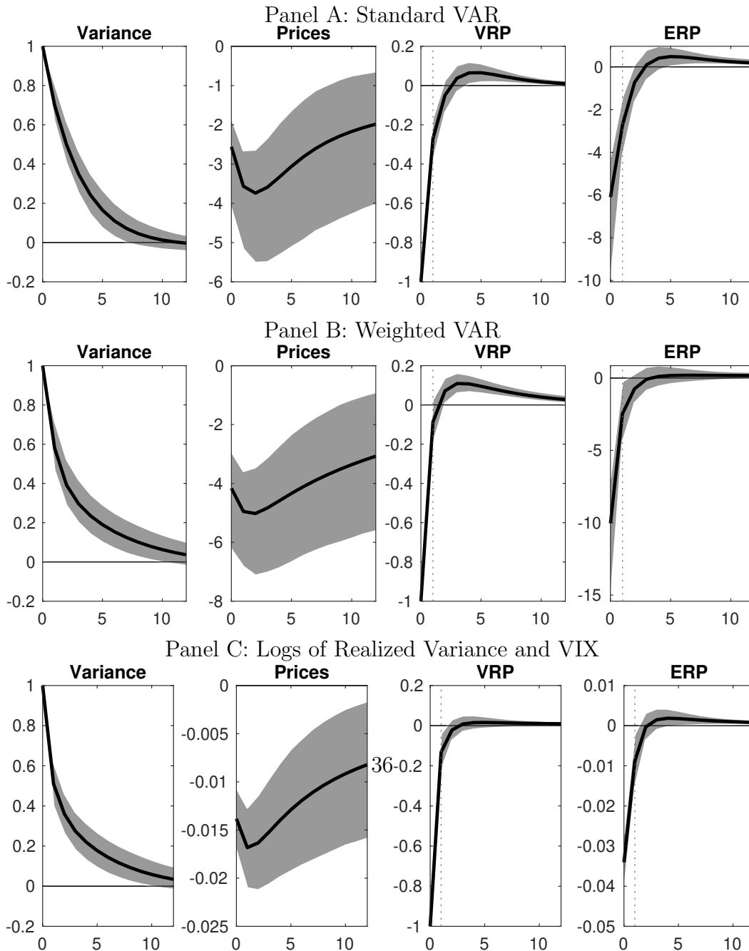
Figure 1: VAR for US data. We run a VAR of realized variance, market excess returns (denoted ERP for equity risk premium), the variance risk premium (VRP), and the log price dividend ratio (labeled Prices). The variance risk premium is implied variance (from the VIX) minus realized variance. We plot the response of each variable to a shock to realized variance at time 0 but also add a vertical dashed line at time 1 to highlight the predicted, rather than realized, equity and variance risk premiums based on the time 0 RV shock. We include the 6 month lag of each variable in the VAR. The x-axis is in months. Confidence intervals are given in the shaded regions. Panel B weights the observations by the inverse of realized volatility (weighted least squares). Panel C uses logs of RV and the VIX in place of levels to downweight outliers. See text for details. Shaded regions indicate 95% confidence intervals constructed using bootstrap. See text for more detail.
